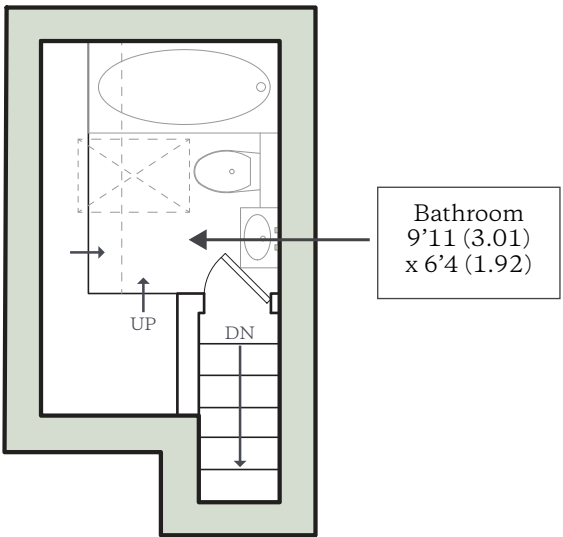
THIRD FLOOR
