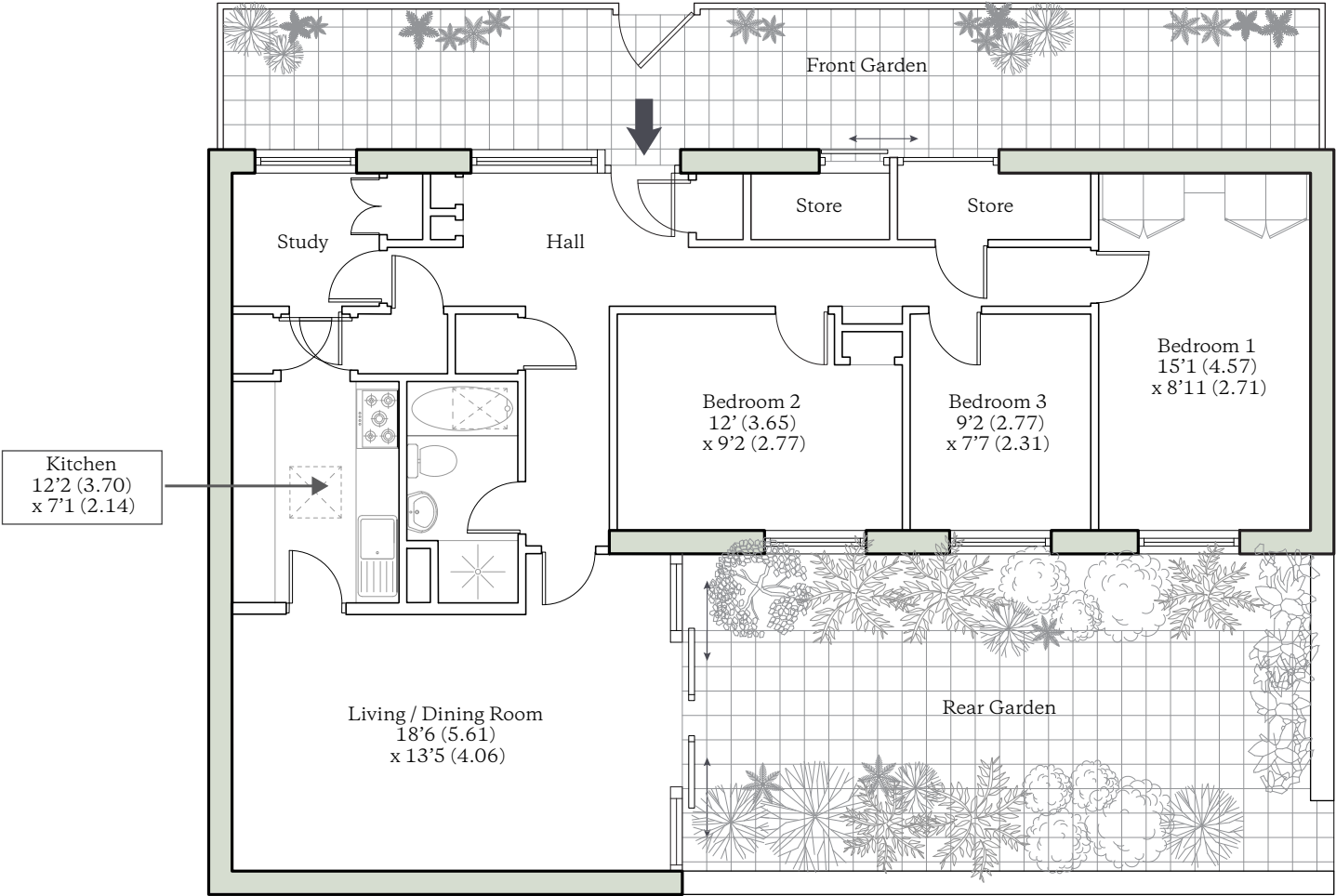
GROUND FLOOR
