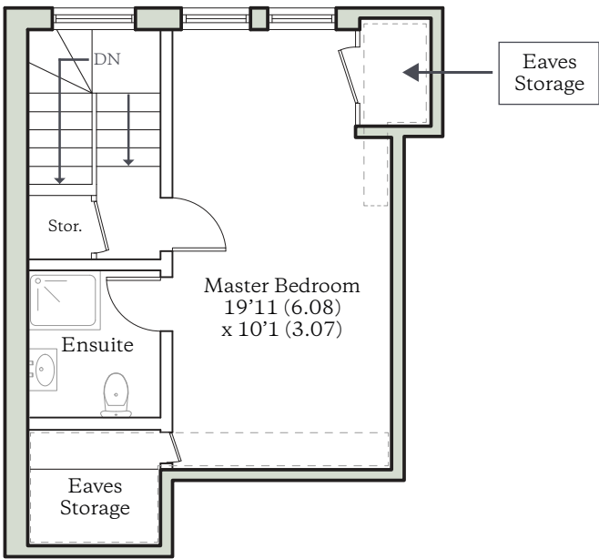
THIRD FLOOR
