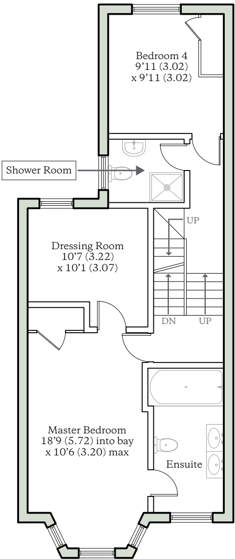
FIRST FLOOR
