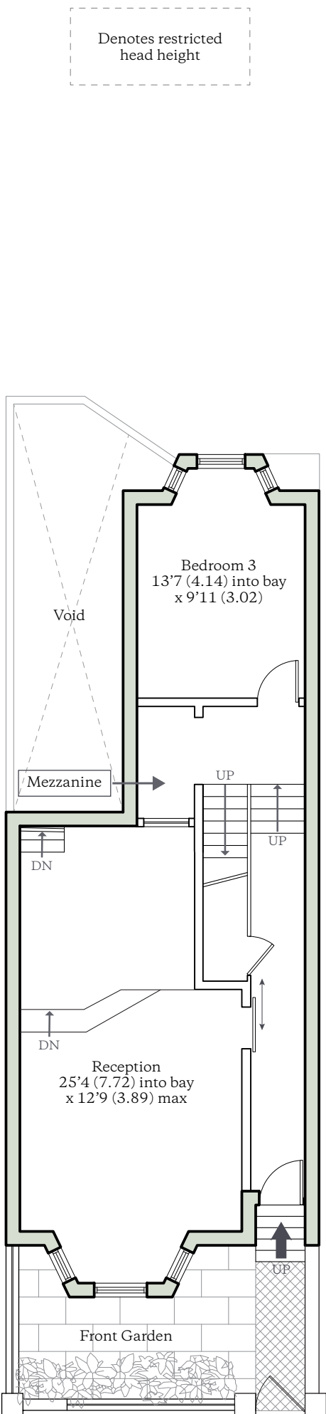
GROUND FLOOR
