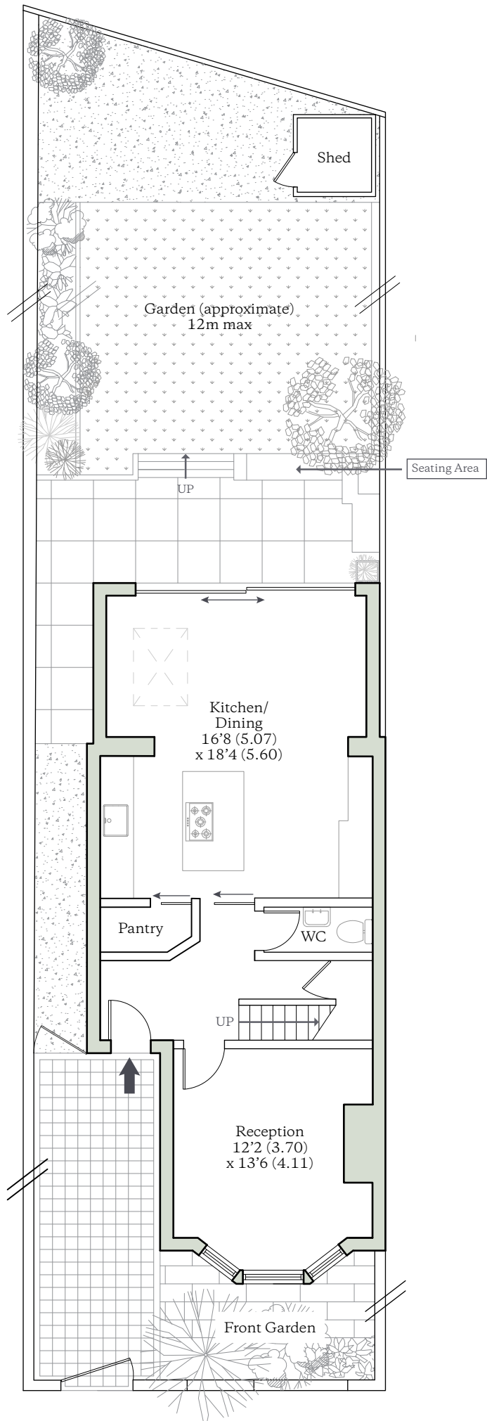
GROUND FLOOR
